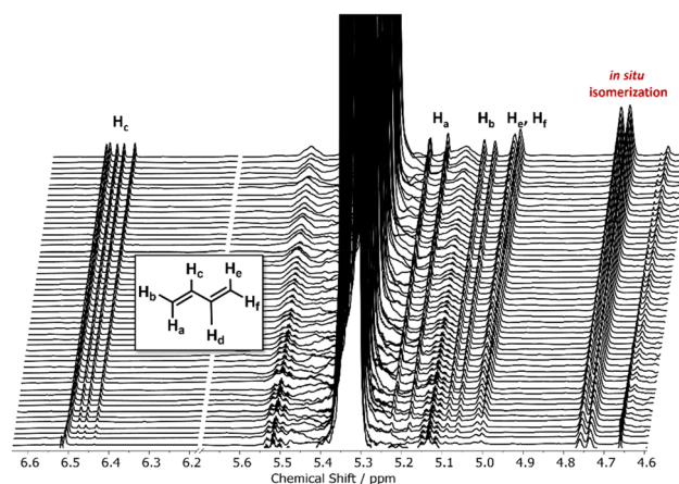
Fig. 3 Zoom-in region of stacked ^1H NMR spectra (400 MHz, THF\text{-}d_8:DMSO\text{-}d_6 = 5:1 ) of the copolymerization kinetic investigation of PreGE and EO, validating the elimination of isoprene in small quantities. The doublet forming between 4.71 and 4.77 ppm shows the concurrent prenyl-to-isoprenyl isomerization under basic AROP conditions.
