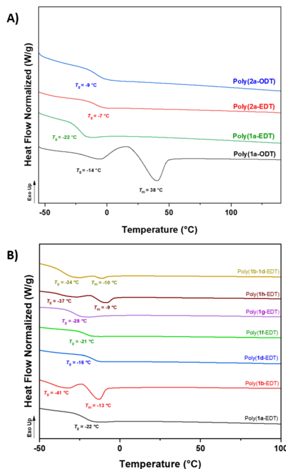
Fig. 2 Thermal properties of OZT-derived thiol–ene polymers. (A): DSC thermograms depicting the second heating cycle between -50 and 150\ ^\circ C of C_{11} and C_5 EDT and ODT polymers. (B) DSC thermograms depicting the second heating cycle between -50 and 100\ ^\circ C of functionalised thiol–ene polymers.
