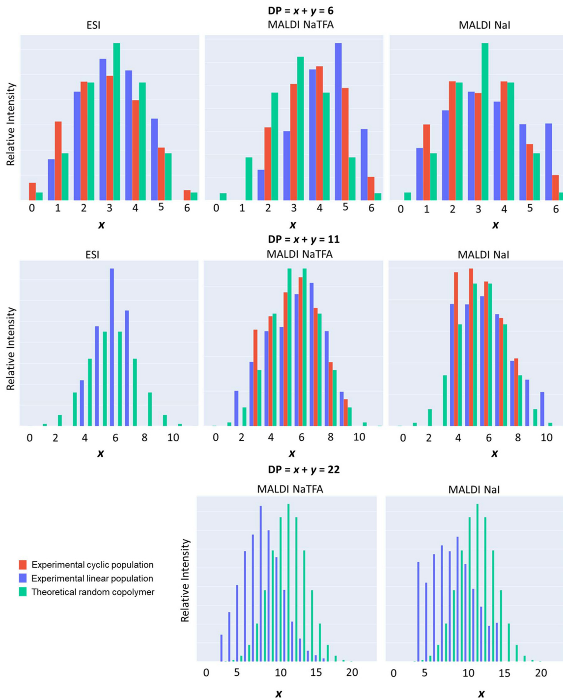
Fig. 7 Histograms of experimental (blue: linear and red: cyclic) macromolecular ion distributions in a P[(\text{CL}^{n\text{Bu}})_x\text{-co-}(\text{CL}^{\text{Me}})_y] copolymer (Table 1, entry 3) for selected \text{DP} = x + y = 6, 11, and 22 extracted from (left) ESI HRMS, (middle) MALDI-ToF MS using \text{CF}_3\text{CO}_2^-\text{Na}^+ , and (right) MALDI-ToF MS using \text{Na}^+\text{I}^- as an ionizing source, and compared to theoretical (green) random copolymer distribution calculated from a binomial law.
