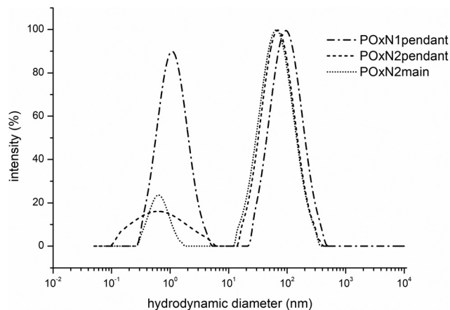
Fig. 3 Distribution of the hydrodynamic diameter (intensity weighted distribution) for aqueous solutions of POxN1pendant, POxN2pendant and POxN2main ( 7.5 \text{ mg mL}^{-1} , 25^\circ \text{C} ).
