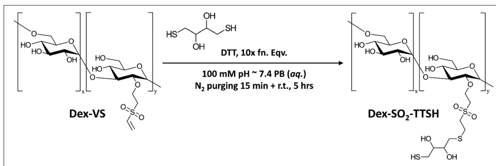
Scheme 2 Synthesis of dextran sulfonyl thiothreitol ( \text{Dex}_{40k}\text{-SO}_2\text{-TTSH} ) utilizing reagent DL-dithiothreitol (DTT) by Michael Addition of thiol ( -\text{SH} ) with sulfonyl-activated vinyl ( -\text{CH}=\text{CH}_2 ) moieties of \text{Dex}_{40k}\text{-VS} in ambient, slightly basic, and low-oxygen condition, with thiol in excess. 27b
