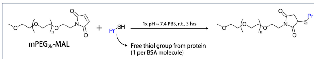
Scheme 3 Synthesis of PEGylated BSA ( \text{mPEG}_{2k}\text{-MALS-BSA} , abbr. pBSA) utilizing reagent poly(ethylene glycol) monomethyl ether maleimide ( \text{mPEG}_{2k}\text{-MAL} ) by Michael Addition of thiol ( -\text{SH} ) with carbonyl-activated vinyl ( -\text{CH}=\text{CH}- ) moieties on the maleimide functional group in ambient and slightly basic condition, with maleimide in excess. 28
