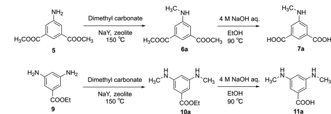
Scheme 1 Synthetic routes of 7a and 11a .
