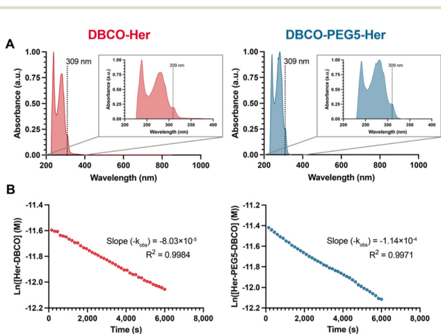
Fig. 5 (A) UV-Vis spectrum of DBCO-Her conjugates in PBS (pH 7.2). (B) Representative linear graph of the natural log of DBCO-Her concentration ( M ) vs. time (s) upon the addition of azide 4 (1 mM). DBCO-Her (2) is represented in red (left panels) and DBCO-PEG 5 -Her (3) in blue (right panels).
