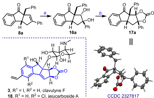
Scheme 5 Elaboration of 8a to the tetracyclic framework of clavulyne and jejucarboside family of natural products. Reagents and conditions: (a) \text{OsO}_4 (10 mol%), NMO (2.5 equiv.), THF : water (5 : 1), RT, 24 h, 90%. (b) CDI (2 equiv.), \text{Et}_3\text{N} (2 equiv.), dry DCM, RT, 6 h, 86%.
