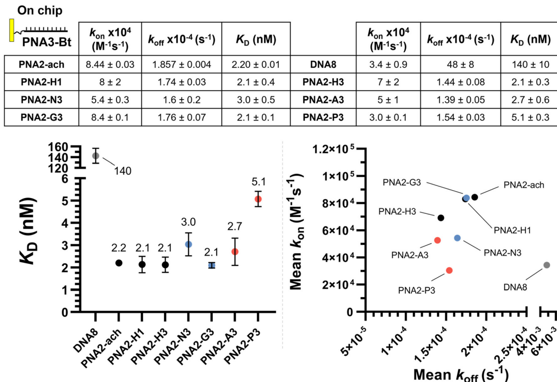
Fig. 4 SPR dissociation equilibrium constants ( K_{\text{D}} ), association rates ( k_{\text{a}} ) and dissociation rates ( k_{\text{d}} ) for PNAs for PNA3-Bt immobilized on the chip. Data presented as the average of duplicate measurements ( n = 2 ) and reported as the mean \pm 95% CI ( z = 1.96 ). Plotted error bars represent the standard deviation (SD).
