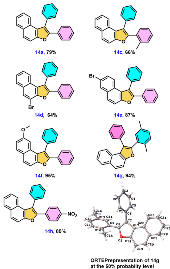
Scheme 5 Synthesis of naphthofurans 14a–14h using various naphthofuranone derivatives 12a , 12b , 12i–12n . Reaction conditions: 0.5 mmol of 12a , 1.25 mmol of LAH, and ether as a solvent (0.5 mL) at 0 °C in N 2 atm, then 0.5 mmol of 13a , 0.5 mmol of triflic acid, and acetonitrile (0.5 mL) as a solvent.
