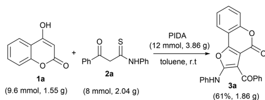
Scheme 2 Gram-scale synthesis of 3a . Reaction conditions: 1a (0.3 mmol), 2a (0.25 mmol), PIDA (1.5 equiv.), BHT (3 equiv.) and solvent (2.0 mL), room temperature in an open atmosphere.
