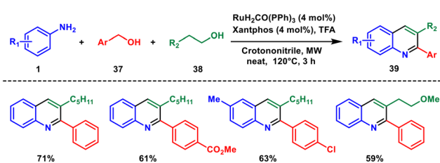
Scheme 14 Ru-catalysed reaction with alkyl and aryl alcohol.
