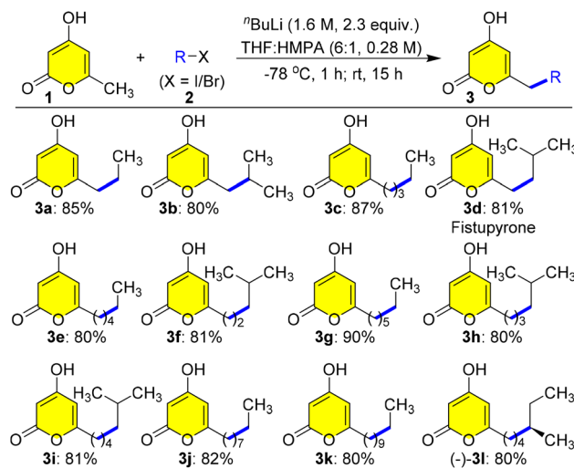
Scheme 2 Synthesis of 7-alkyl-4-hydroxy-2 H -pyran-2-ones 3 from triacetate lactone 1 . Reaction conditions: the reaction mixture of 1 (5.0 mmol) in THF/HMPA (6 : 1, 17.5 mL) with n BuLi (1.6 M, 2.3 equiv.) at -78 °C was stirred for 1 h before addition of alkyl halide 2a–l (2.0 equiv.) followed by stirring at rt for 15 h. Yields refer to the column purified products.
