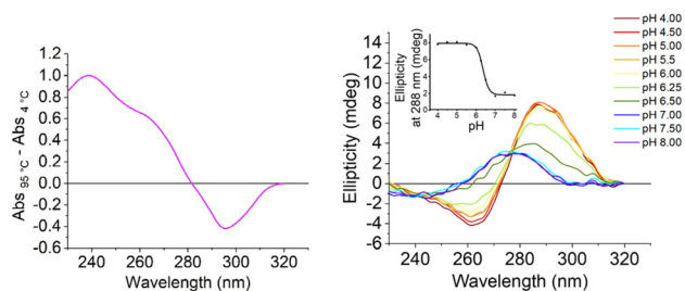
Fig. 2 Left: thermal difference spectra of the C-rich i-motif forming S100P sequence: at 2.5 \mu\text{M} in 10 mM lithium cacodylate and 100 mM KCl buffer at pH 5.5. Right: CD spectra of the C-rich S100P sequence at 10 \mu\text{M} DNA in 10 mM lithium cacodylate and 100 mM KCl buffer at pH as indicated. Inset: corresponding plot of ellipticity at 288 nm at the different pHs to determine the transitional pH.
