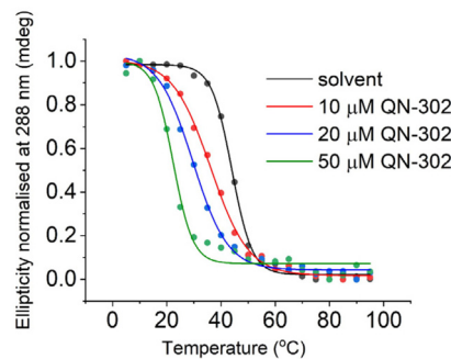
Fig. 3 Representative CD melting experiments with 10 \mu\text{M} S100P i-motif in 10 mM lithium cacodylate 100 mM KCl buffer (pH 5.5), and 0, 10, 20 or 50 \mu\text{M} QN-302, as indicated.
