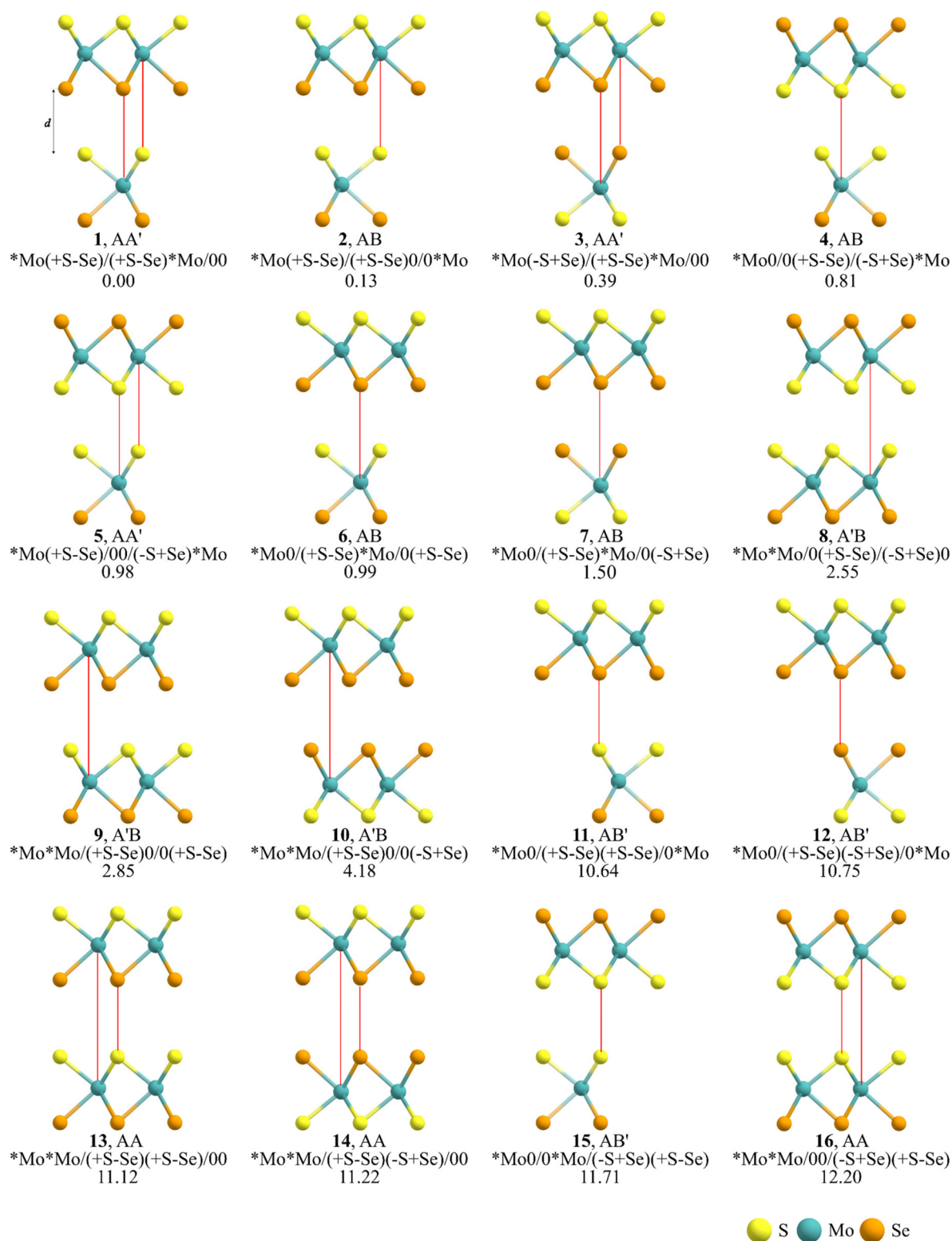
Fig. 4 JAM strings of the sixteen stacking configurations of bilayer MoS 2 Se. Relative energies (ΔE) in meV per atom computed at the SCAN-rVV10 level. Red lines indicate eclipsed atoms.
