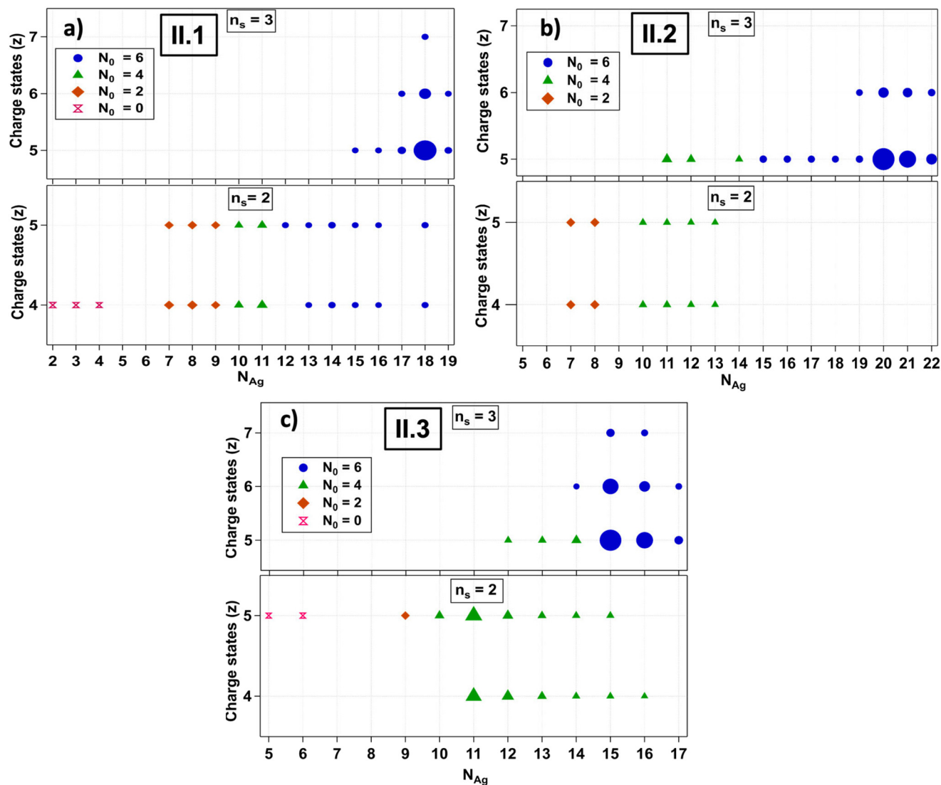
Fig. 3 Transition of N_0 with N_{Ag} for Group II Ag_N -DNAs: (a) II.1, (b) II.2, and (c) II.3. Peaks containing N_0 = 6, 4, 2, and 0 are denoted with blue circles, green triangles, ochre diamonds, and pink double triangles, respectively. Species stabilized by three and two DNA oligomers ( n_s = 3 and 2 ) are detected.
