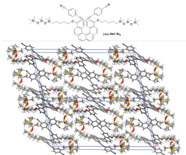
Fig. 4 Chemical structure and supramolecular assembly of 2,15-bis-cyanophenyl-carbo[6]helicene-siloxane adduct rac -Hel'-Si 3 obtained from X-ray data analysis.
