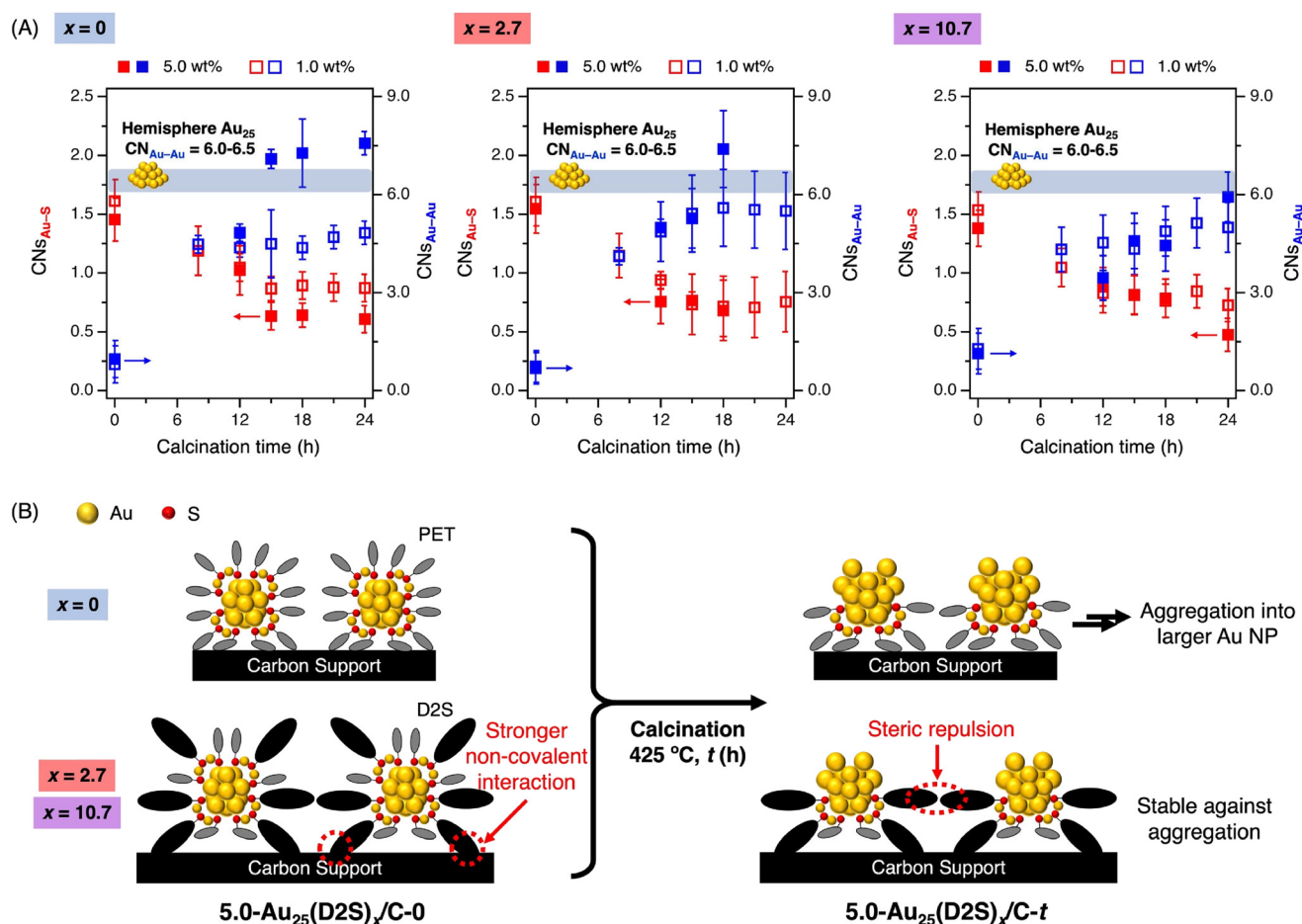
Fig. 2 (A) Time course of \text{CN}_{\text{Au-S}} (red) and \text{CN}_{\text{Au-Au}} (blue) of w\text{-Au}_{25}(\text{D2S})_x/\text{C}-t with x = 0, 2.7, and 10.7 estimated from curve fitting analyses of Au L_3 -edge EXAFS oscillations. Blank and filled squares correspond to the data for w = 1.0 and 5.0 , respectively. (B) Schematic representation of the ligand desorption from 5.0\text{-Au}_{25}(\text{D2S})_x/\text{C} and the model structures of 5.0\text{-Au}_{25}(\text{D2S})_x/\text{C}-t .
