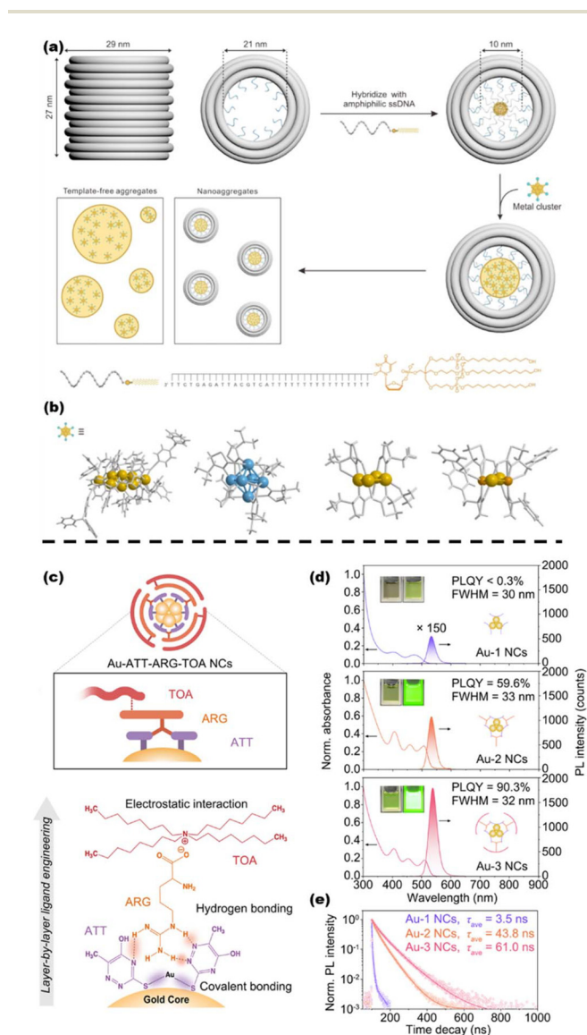
Fig. 8 (a) Design and operation of a hydrophobic alkyl core barrel DNA framework, as well as a schematic representation of the polymerization of MNCs directed by a DNA framework. (b) MNCs employed in the study and their atomic structures. \text{Au}_8 , \text{Ag}_6 , \text{Au}_4 , and \text{Au}_2\text{Cu}_2 are arranged from left to right. Reproduced from ref. 168 with permission from the American Chemical Society, copyright (2024). (c) Schematic illustration of the layer-by-layer self-assembly evolution of triple-ligands. ATT = purple, ARG = orange, and TOA = pink. (d) UV-vis and photoluminescence spectra of Au-1, Au-2, and Au-3 nanoclusters, the insets show the digital optical photographs of Au-1, Au-2, and Au-3 under ambient conditions (left) and 365 nm excitation (right). (e) Luminescence time-resolved spectra of Au-1, Au-2, and Au-3 under 405 nm excitation. Reproduced from ref. 170 with permission from Springer Nature, copyright (2023).
