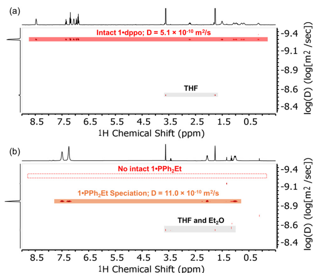
Fig. 3 ^1\text{H} DOSY NMR spectra ( \text{THF-d}_8 , 400 MHz) of (a) 1-dppo and (b) 1-PPh 2 Et showing the unique ability of the dppo ligand to arrest speciation of the [\text{Cu}_{12}\text{S}_6] cluster core. Dashed line in (b) indicates the calculated diffusion coefficient for intact 1-PPh 2 Et based on the crystallographic structure. 61
