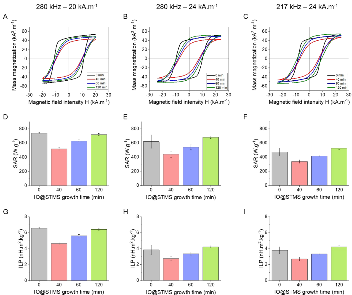
Figure 10: A), B) and C) Representative hysteresis cycles for the different IO@STMS-t NPs (IO@STMS-0 and for IO@STMS-t (t=40,60,120 min)) obtained from series 2 at different frequency-amplitude conditions. D), E) and F) Corresponding SAR values. G), H) and I). Corresponding ILP values.
