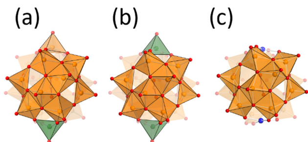
Fig. 1 Anion structures of (a) V18ox, (b) V18, and (c) \text{Cu}_2\text{V16} . Orange and green square pyramids represent \text{V}^{5+}\text{O}_5 and \text{V}^{4+}\text{O}_5 . Red and blue spheres represent oxygen and copper atoms. The deep and pale colours of the \text{V}^{5+}\text{O}_5 units represent front and back sides. Nitrate locates at the centre of the clusters.
