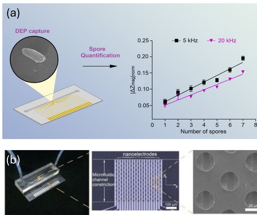
Figure 21: (a-b) A microfluidic device comprising 190 microwells and 20 aluminium nanoelectrodes adapted for performing dielectrophoresis (DEP) to capture spore, and the results of individual electrochemical impedance spectroscopy (EIS) measurements is shown in the line plot on right, enabling precise quantification. Reprinted with permission from ref. (89) (copyright open access © 2021 Published by American Chemical Society).
