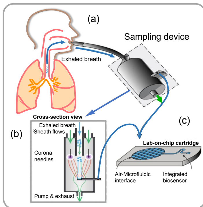
Figure 17: (a) Schematic illustration of a point-of-care (PoC) system designed for sampling aerosol from a high-volume of air directly into a microfluidic device that captures exhaled breath condensate, (b) sampling device cross-sectional view integrated with a microfluidic detector, (c) a lab-on-chip cartridge with a microfluidic interface that allows diagnosis from an exhaled-breath aerosol (86).
