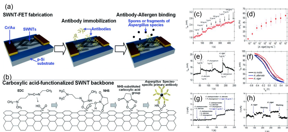
Figure 13: (a) illustration of the antibody-allergen binding and the fabrication of fungi sensors based on SWNT-FETs for binding of allergens (b) EDC/NHS chemistry was utilized to immobilize WF-AF-1 Abs directly onto the carboxylic acid-functionalized SWNT surface (c) The real-time response of an SWNT-FET device immobilized with WF-AF-1 Abs to a series of injections of varying concentrations of A. niger -suspended PBS solution (d) corresponding calibration curve (e) response of the functionalized SWNT-FET device in real-time to a random
