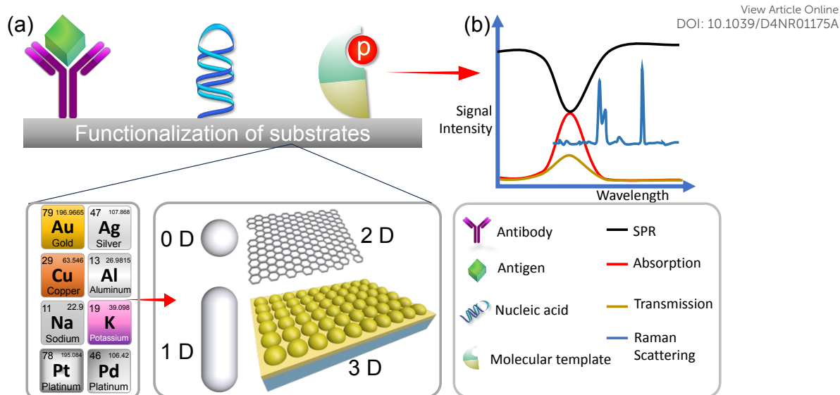
Figure 2: (a) Demonstrates the functionalization process of the substrate with various optical materials and the attachment of specific receptors for enhancement of sensitivity and specificity (b) Depicts the signal detection mechanism, involving the selection of modes such as Surface Plasmon Resonance (SPR), Absorbance, Transmission or Raman Scattering, enabling precise analyte detection and analysis.
