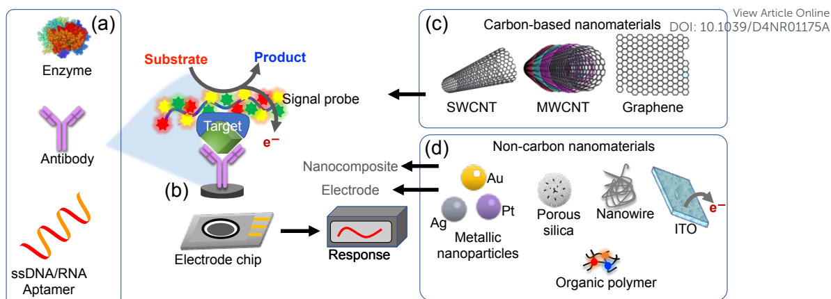
Figure 10: Schematic diagram of an electrochemical sensor: (a) biological recognition elements such as those but not limited to antibodies, enzymes, or DNA are designed for target specificity; (b) these elements are applied onto the working electrode, (c-d) materials that enhance the electrochemical signals that have been used to modify the working electrodes such as carbon and non-carbon materials such as SWCNT, MWCNT, graphene, NPs, polymers, or nanowires. The transducer converts biochemical signals into electrical signals, facilitating accurate measurement and analysis (69).
