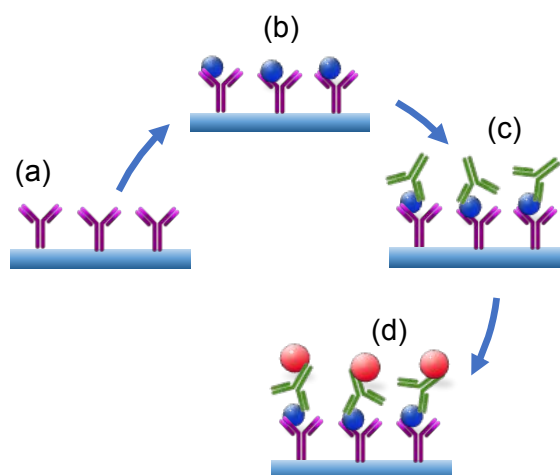
Figure 15: The schematic representation of the magneto-nanosensor biochip immunoassay involves several steps (a-b) immobilization of antibodies on the surface of the working electrode (c) sandwich structures are formed through the addition of biotinylated detection antibodies (d) magnetic nanoparticles bound to the detection antibodies generate a stray magnetic field that results in a change in sensor resistance due to the GMR effect (72).
