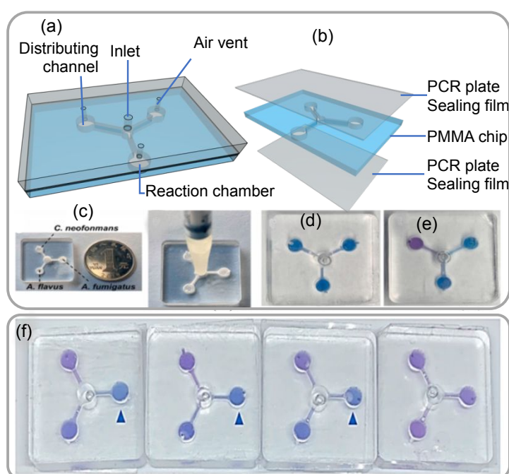
Figure 18: (a) Description of the apparatus (b) assembly of the chip (c) three sets of primers were preloaded with 0.5% low melt agarose in the reaction chamber (d) The chip's adapter (e) Verification of the possibility and cross-contamination of LAMP assays implemented on the microfluidic chips (f) Outcomes of the colorimetric LAMP assays conducted on the chips at 4 \times 10^6 , 4 \times 10^5 , 4 \times 10^4 and 4 \times 10^3 spores per sample. Reprinted with permission from ref. [50] (copyright © 2022 Published by Elsevier B.V.).
