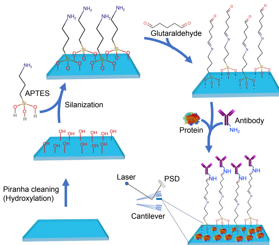
Figure 16: Scheme showing silicon microfabricated cantilever functionalization by treating the surface with APTES, glutaraldehyde followed by covalent attachment of anti- Aspergillus niger polyclonal antibodies ~IgG designed to capture fungal spores (73). Binding of spores to
