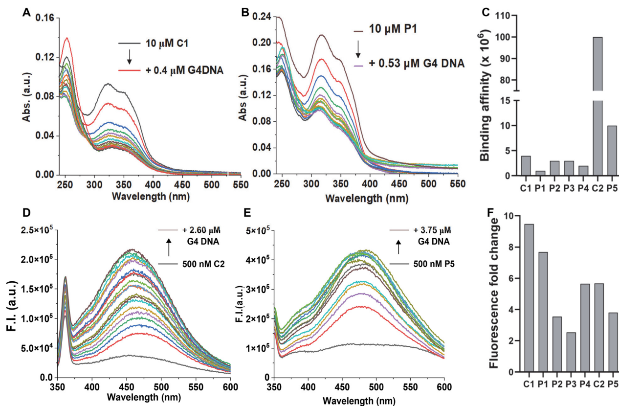
Fig. 5 UV-Vis titration spectra of 10 \mu M ligands (A) C1 and (B) P1 , and (C) binding affinities for all the molecules in 10 mM Tris-HCl (pH 7.4), 0.1 mM EDTA and 0.1 M KCl with 10 \mu M pre-formed Hum 21-mer G4 DNA. Fluorescence titration spectra of 0.5 \mu M ligands (D) C2 and (E) P5 , and (F) fold-change for all the molecules in 10 mM Tris-HCl (pH 7.4), 0.1 mM EDTA and 0.1 M KCl with 10 \mu M pre-formed Hum 21-mer G4 DNA.
