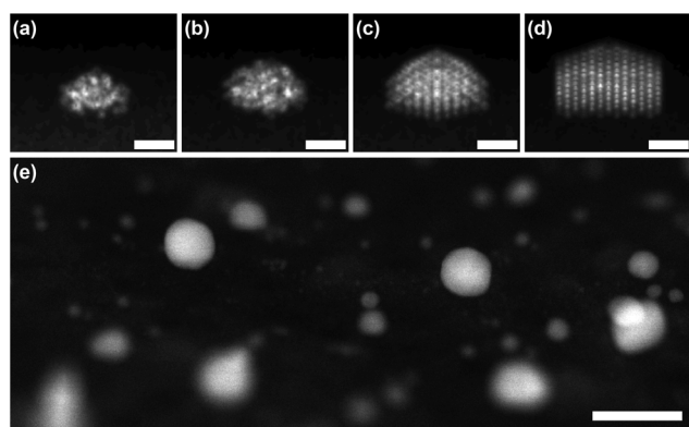
Fig. 2 Comparison of HAADF-STEM simulations of hemispherical truncated clusters on carbon at -70^\circ to experimental data. (a) -70^\circ projection of amorphised hemispherical Au147 icosahedron. (b) -70^\circ projection of amorphised hemispherical Au309 decahedron. (c) -70^\circ projection of hemispherical Au509 decahedron. (d) -70^\circ projection of hemispherical Au923 truncated octahedron. (e) Wide field-of-view experimental HAADF-STEM image acquired at -70^\circ showing all clusters under 1000 atoms in size are approximately spherical. (a–d) Scale bar of 1 nm. (e) Scale bar of 20 nm.
