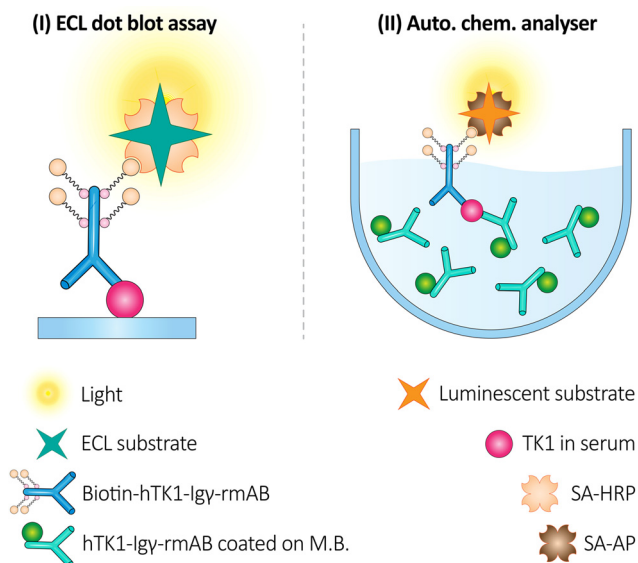
Fig. 14 The scheme illustrates two assays for detecting hTK1 using recombinant monoclonal antibodies (rmAb). The first panel (I) shows an ECL dot blot assay for hTK1 identification using hTK1-IgY-rmAb coated on MBs. The second panel (II) depicts an automated chemiluminescence analyzer using the same antibodies for hTK1 detection in serum. These methods provide sensitive detection of hTK1, a potential biomarker for cell proliferation. Reproduced from ref. 200 under the terms and conditions of the Creative Commons Attribution (CC BY) license ( https://creativecommons.org/licenses/by/4.0/ ).
