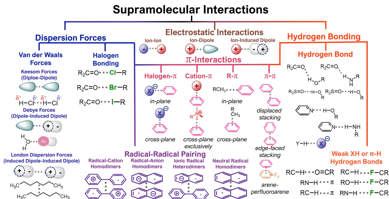
Fig. 3 Supramolecular interactions present in organic molecules electrodes. Adapted from Roman A. Valiulin Copyright © 2020 adapted with permissions from ref. 33. Copyright © 2021 Springer Nature Limited.
