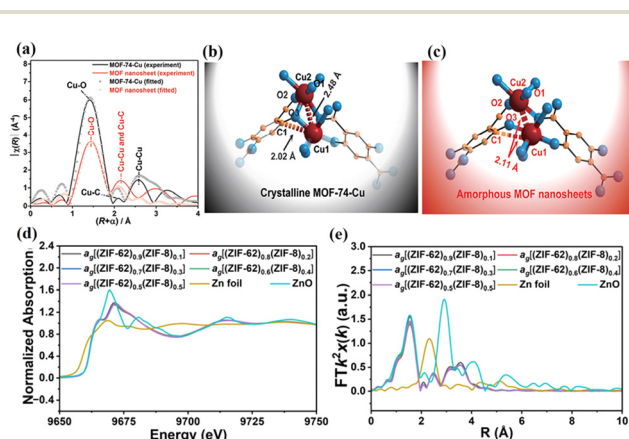
Fig. 4 (a) EXAFS spectra of MOF crystals and nanosheets. Suggested structures of (b) MOF crystals and (c) nanosheets deduced from the analysis of EXAFS. Reproduced with authorisation from ref. 54 and copyright 2021 by The Royal Society of Chemistry. (d) Normalized XANES spectra and (e) EXAFS R-plots of MOF CGC membranes. Reproduced with authorisation from ref. 45 and copyright 2023 by Wiley-VCH GmbH.
