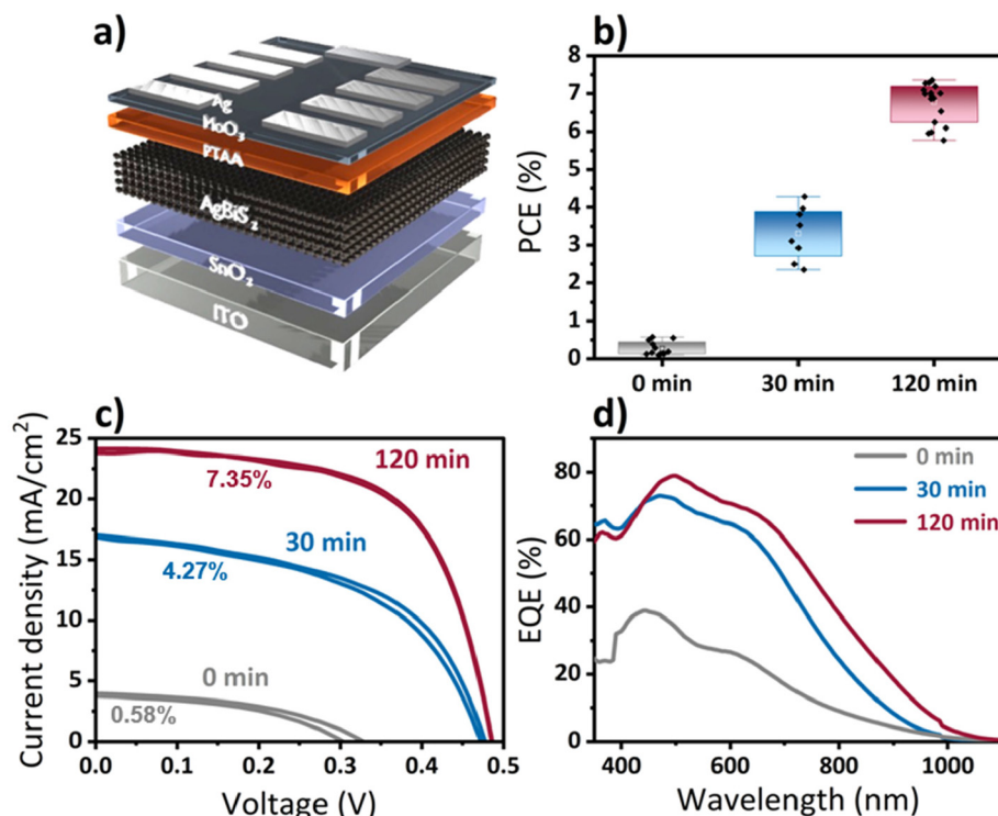
Fig. 5 (a) Schematic device architecture of \text{AgBiS}_2 solar cells, (b) Solar cell performance (PCE) of \text{AgBiS}_2 QDs obtained after different times of cation exchange, (c) J–V curves (forward and reverse scanning) of devices with different QDs after 0 min ( \text{Ag}_2\text{S} ), and \text{AgBiS}_2 after 30 min, and 120 minutes of cation exchange with individual PCE (d) corresponding EQE curves for these three devices.
