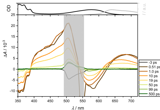
Fig. 4 Transient absorption spectra of the ligand 2 in DCM following excitation at 575 nm (OD = 0.2) were probed between 350 and 720 nm at the indicated delay times (bottom). A distinct grey area, located around 530 nm, is included in the figure to mask the spectral region affected by scattering effects from the excitation pulse. The top section shows the normalized steady-state absorption (black) and emission spectra ( \lambda_{\text{ex}} = 500 nm, slit width 4 nm, grey).
