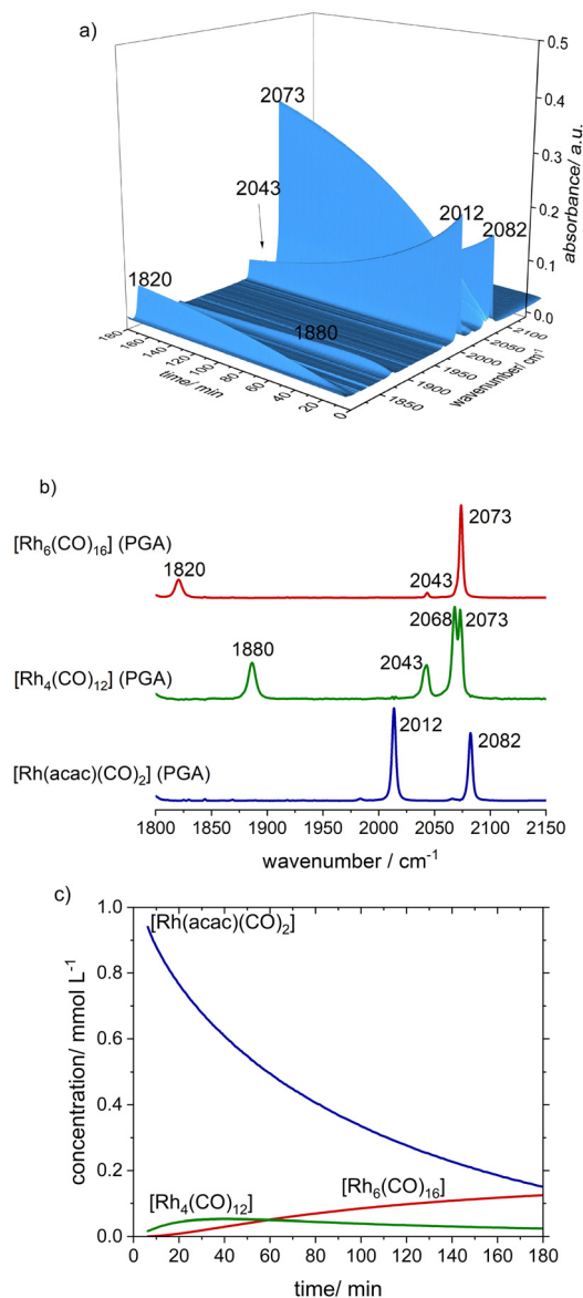
Fig. 4 (a) In situ FTIR-spectra series obtained from the treatment of [\text{Rh}(\text{acac})(\text{
