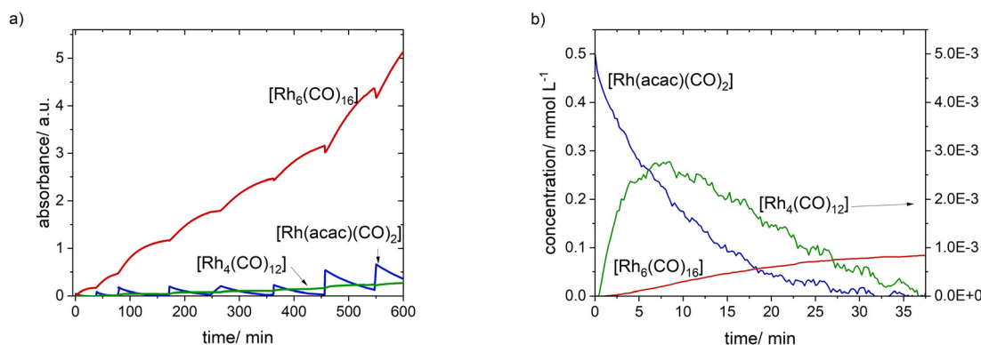
Fig. 3 Extracted profiles of the complexes for the perturbation experiment. (a) Non-scaled absorption- vs. -time profiles for the complete data set; (b
