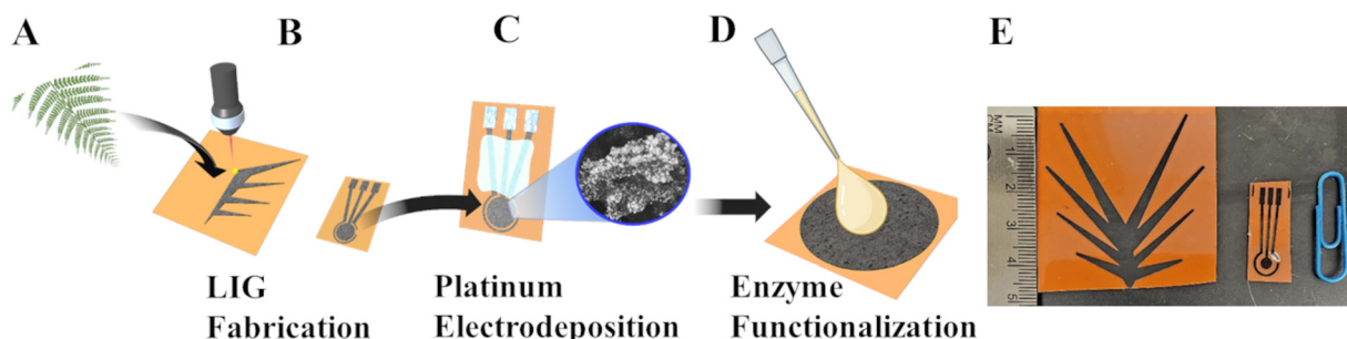
Fig. 1 Fabrication and functionalization schematic of the LIG leaf and electrochemical biosensor. Schematic images demonstrate the (A) fern leaf inspiration, (B) polyimide conversion to LIG using a CO 2 laser to create both the fern leaf pesticide collection patch and the 3-electrode electrochemical biosensor, (C) surface modifications including the electrodeposition of PtNPs onto the LIG working electrode, (D) functionalization of the LIG sensor with the enzyme glycine oxidase for selective glyphosate monitoring, (E) and an optical image of the completed LIG leaf and biosensor. Both a metric scale ruler and a standard no. 1-sized paperclip serve as measurement legends in (E).
