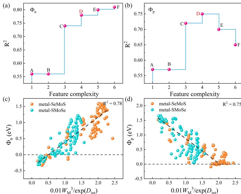
Fig. 8 Pareto chart of R^2 for (a) \Phi_n and (b) \Phi_p vs. complexity of the proposed mathematical formulas. The correlations of the calculated (c) \Phi_n and (d) \Phi_p values of metal–MoSSe contacts vs. predicted 0.01W_M^3/\exp(D_{\text{int}}) formula from SISSO. The data here are all derived from the DFT calculation results in this work.
