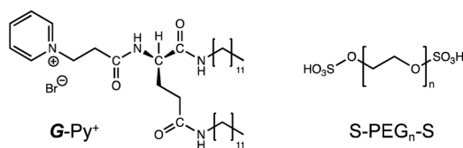
Scheme 1 Chemical structures of glutamide-derived lipid with pyridinium head group ( G\text{-Py}^+ ) and termini-anionised hydrophilic polymer ( S\text{-PEG}_n\text{-S} ).
