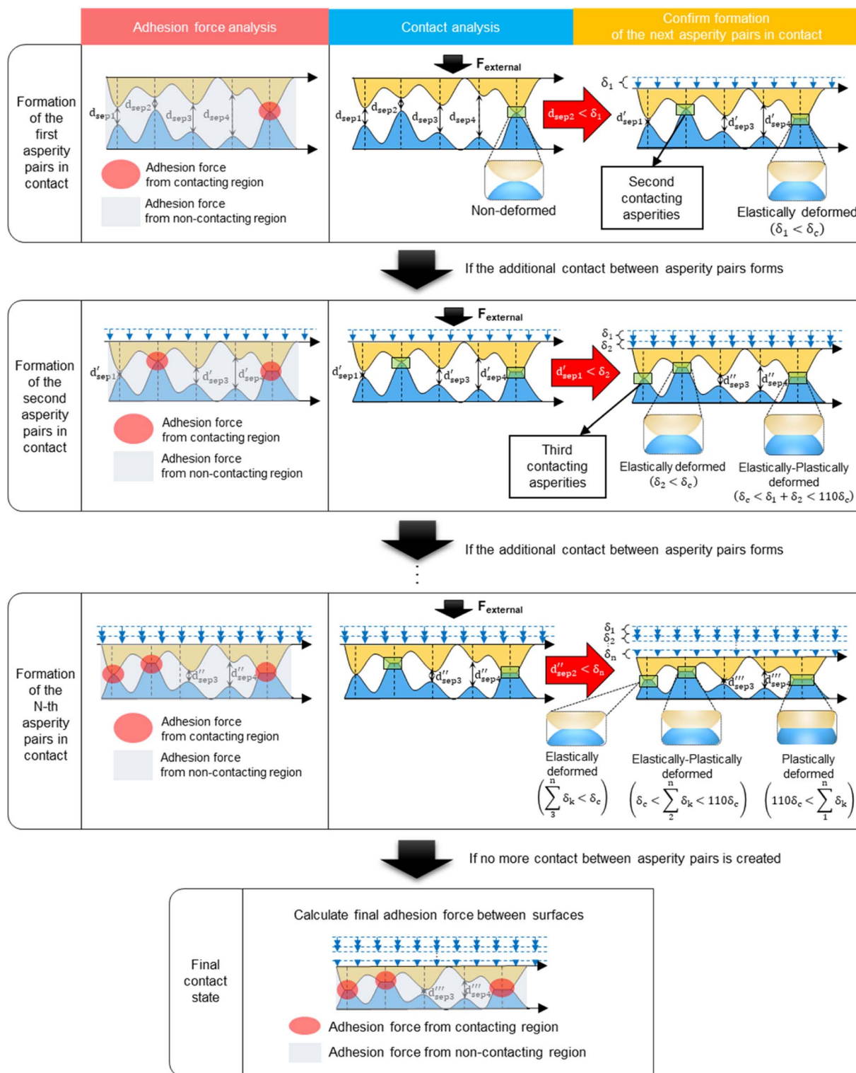
Fig. 2 Iteration process for simulating the real contact process. In the iteration process, the process of adhesion force analysis, contact analysis, and determination of the next contact between asperities is repeated until the final separation distance is reached. The schematics demonstrate the iterative analytical process of our model from the very first formation of the asperity pairs to the last, when no more new asperity pairs are created due to compressive densification of the contact interface. The aforementioned iterative processes are performed sequentially and repetitively with every new formation of asperity pairs. In the adhesion force analysis, an appropriate adhesion model is determined and utilized based on the contact condition of each of the asperity pairs. In the contact analysis, the extent of deformation between asperity pairs covering both elastic and plastic deformation is analyzed based on the calculated adhesion force from the previous adhesion force analysis and the external force applied between each contact surface. Based on the amount of deformation, our model determines whether additional contact between asperities can be made and more iteration is necessary based on the degree of deformation between existing asperity pairs in contact and the remaining separation distance of the non-contacting asperities.
