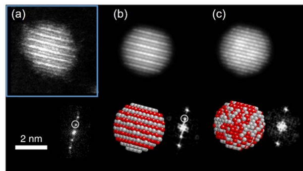
Fig. 7 (a) STEM-HAADF image of one Ag/Pt NP oriented along the [011] zone axis showing L1_1 phase with alternating planes of Ag and Pt and its corresponding FFT showing the superstructure reflections (marked with white circle). In the HAADF image, Pt atom columns are brighter than Ag atom columns, for Pt has a higher atomic number than Ag. (b and c) Simulated STEM-HAADF images along [011] zone axis for an L1_1 structure and a random solid solution, respectively. Adapted from ref. 97 under CC BY license @ 2019, the Author(s). Copyright 2019, Springer Nature.
