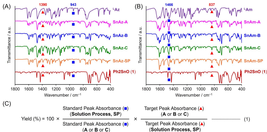
Fig. 1 FT-IR spectra of (A) L\text{-Az} , \text{SnAz-A} , B, C and SP, and \text{Ph}_2\text{SnO} (1), (B) L\text{-Am} , \text{SnAm-A} , B, C and SP, and \text{Ph}_2\text{SnO} (1). (C) Chemical formula for calculating the yields of mechanochemical reactions under various conditions. Square and triangle marks denote standard peaks and target peaks, respectively. Standard peak: originating from both the precursor ( L\text{-Az} or L\text{-Am} ) and the products (A, B, C, and solution process, SP). Target peak: originating only from product (A, B, C, and solution process, SP). \text{Ph}_2\text{SnO} (1) has neither standard peaks nor target peaks.
