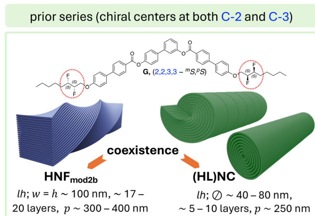
Fig. 2 Bent-core molecule with chiral centers at C-2 and C-3 via the introduction of ( S,S )-2,3-difluorooctyloxy side chains (compound G ): 27 upon slow as well as rapid cooling, G showed a coexistence of two morphologies (HNF mod2b ) and (HL)NC; heliconal layering was here only observed for some of nanocylinders (unlike for compound D ; Fig. 1, which showed heliconal layering depending on the configuration of the chiral center).
