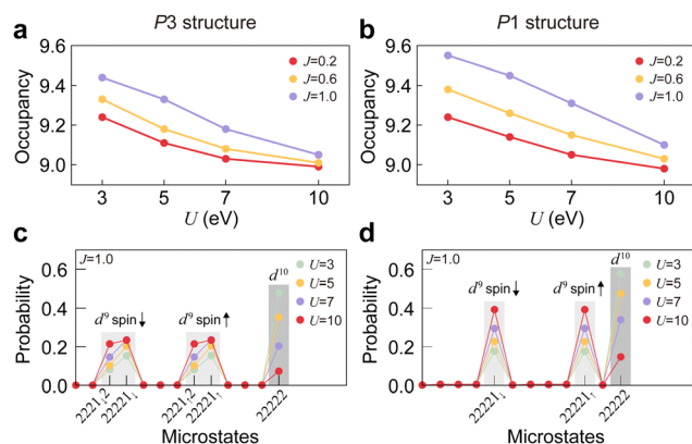
Fig. 5 Occupancy of copper d orbitals and their valence histogram. (a) and (b) Occupancy of copper d orbitals as a function of U and J for the P3 structure and (b) the P1 structure. (c) and (d) Valence histogram as a function of U ( J = 1 eV) for (c) the P3 structure and (d) the P1 structure. 22221 1 refers to the d^9 electron configuration of copper, where the first four orbitals are fully occupied (denoted as 2), and the fifth orbital is half occupied by a spin-up electron (denoted as 1 1 ). The orbital sequence is \{d_{z^2}, d_{x^2-y^2}, d_{xy}, d_{xz}, d_{yz}\} for the P3 structure and \{d_1, d_2, d_3, d_4, d_5\} for the P1 structure.
