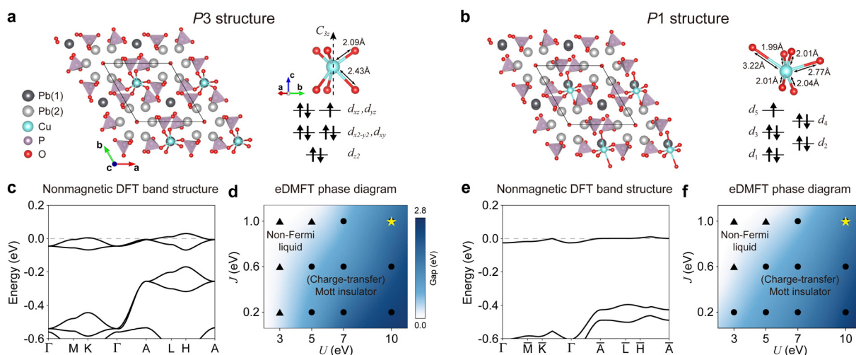
Fig. 1 Crystal structures, electronic structures, and correlation phase diagrams of copper-doped lead apatite. (a) and (b) Crystal structures of Pb 9 Cu(PO 4 ) 6 O with a P 3 space group and P 1 space group. (c) DFT band structure for the P 3 structure. (d) eDMFT phase diagram in the Hubbard U and Hund's coupling J parameter spaces for the P 3 structure. (e) DFT band structure for the P 1 structure. (f) eDMFT phase diagram in the U and J parameter spaces for the P 1 structure. In (d) and (f), the color bar indicates the Mott gap near the Fermi level. Triangles represent metallic states, while circles represent insulating states. The star indicates the constrained eDMFT values of U and J .
