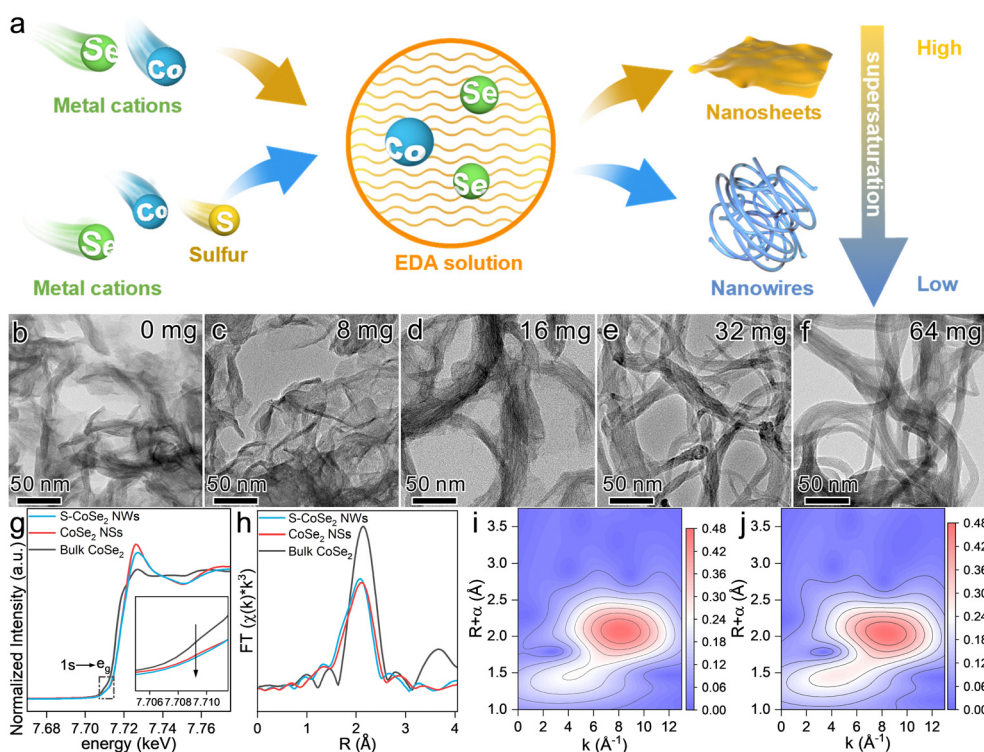
Fig. 2 (a) Formation mechanism of \text{CoSe}_2 NSs and S-CoSe 2 NWs. (b)–(f) Morphological evolution of \text{CoSe}_2 materials with different sulfur contents. (g) Co K-edge XANES spectra and (h) corresponding Fourier transforms of k^3 -weighted EXAFS spectra for \text{CoSe}_2 materials. Wavelet transforms of k^3 -weighted EXAFS spectra of the Co K-edge for (i) \text{CoSe}_2 NSs and (j) S-CoSe 2 NWs.
