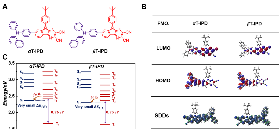
Fig. 1 (A) The chemical structures of \alpha T-IPD and \beta T-IPD. (B) HOMO and LUMO, and T_1 states spin-density distributions (TSDDs) of \alpha T-IPD and \beta T-IPD, respectively. (C) Calculated energy arrangement of singlet states and triplet states of \alpha T-IPD and \beta T-IPD.
