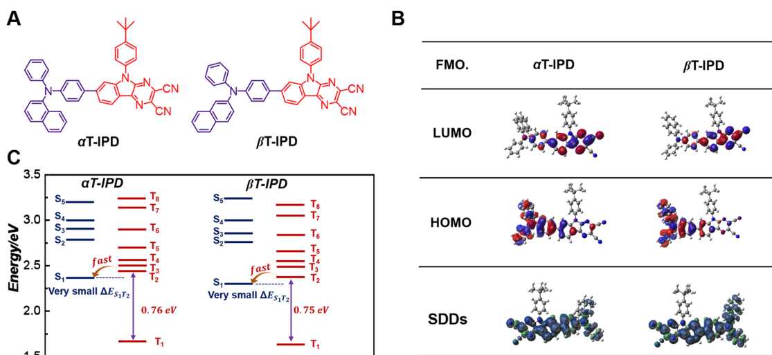
Fig. 1 (A) The chemical structures of \alpha T-IPD and \beta T-IPD. (B) HOMO and LUMO, and T_1 states spin-density distributions (TSDs) of \alpha T-IPD and \beta T-IPD, respectively. (C) Calculated energy arrangement of singlet states and triplet states of \alpha T-IPD and \beta T-IPD.
