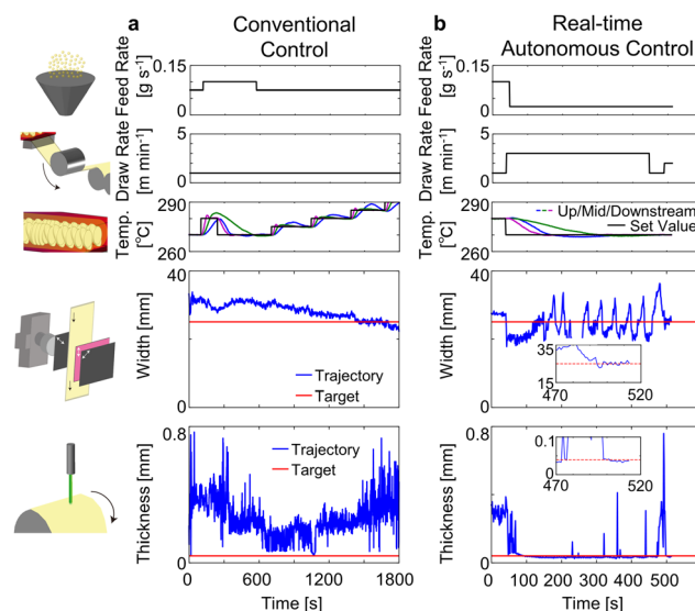
Fig. 2 Effects of autonomous control. Comparison of time-series profiles of feed rate, draw rate, temperature, and film properties (width, thickness) under (a) conventional and (b) autonomous control.
