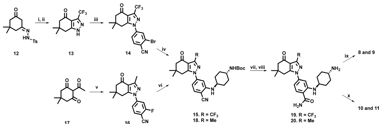
Scheme 1 i) (\text{CF}_3\text{CO})_2\text{O} , TNF, \text{NEt}_3 , 55\text{ }^\circ\text{C} , 2 h; ii) NaOH, MeOH, \text{H}_2\text{O} , r.t., 3 h, 45%; iii) 2-bromo-4-fluorobenzonitrile, NaH, anhy. DMSO, 45\text{ }^\circ\text{C} , 40 h, 57%; iv) trans - N -Boc-1,4-cyclohexanediamine, \text{DPPF}[\text{PdCl}_2] , DPPF, \text{NatOBu} , THF, 65\text{ }^\circ\text{C} , 65%; v) 2-fluoro-4-hydrazinylbenzonitrile, MeOH, AcOH, r.t., 3 d, 67%; vi) trans - N -Boc-1,4-cyclohexanediamine, DIPEA, DMSO, 90\text{ }^\circ\text{C} , 60 min, 74%; vii) EtOH, NaOH, 30% \text{H}_2\text{O}_2 , \text{H}_2\text{O} , r.t., 16 h, 60%. viii) TFA, DCM, r.t., 5 h, 41–79%. ix) 6-Phosphonohexanoic acid, DIPEA, EDCI, NHS, DMF, r.t., 42 h, 53–62%; x) 4-bromo-1-butan-1-ylsulfonic acid, DIPEA, DMF, 50\text{ }^\circ\text{C} , 18 h, 39–52%.
