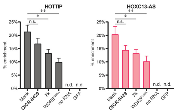
Fig. 3 iv -RIP results using RNA isolates from U-2 OS cells and WDR5 WT , WDR5 F266A , or GFP. Compounds OICR-9429 and 7k were tested at 10 μM in combination with WDR5 WT . The no RNA control was tested with WDR5 WT . n.s.: p > 0.05 , *: 0.05 \geq p > 0.01 , **: 0.01 \geq p > 0.001 .
