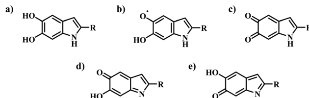
Fig. 1 The monomer building blocks of eumelanin. (a) 5,6-Dihydroxyindole (DHI) for R=H or 5,6-dihydroxyindole-2-carboxylic acid (DHICA) for R=COOH . (b) Protonated semiquinone. (c) Quinone. (d) Quinone imine tautomer. (e) Quinone methide tautomer.
