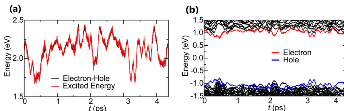
Fig. 5 (a) Time evolution of the many-body electronic excitation energy, including excitonic binding (red), in a 2 \times 2 \times 2 supercell nonadiabatic quantum molecular dynamics (NAQMD) simulation, along with compared energy difference between the electron and hole (black). (b) Time evolution of KS eigen energies, with the KS states that mostly contribute to the quasi-electron and quasi-hole shown in red and blue, respectively. Adapted from ref. 85, Copyright 2016, Springer Nature.
