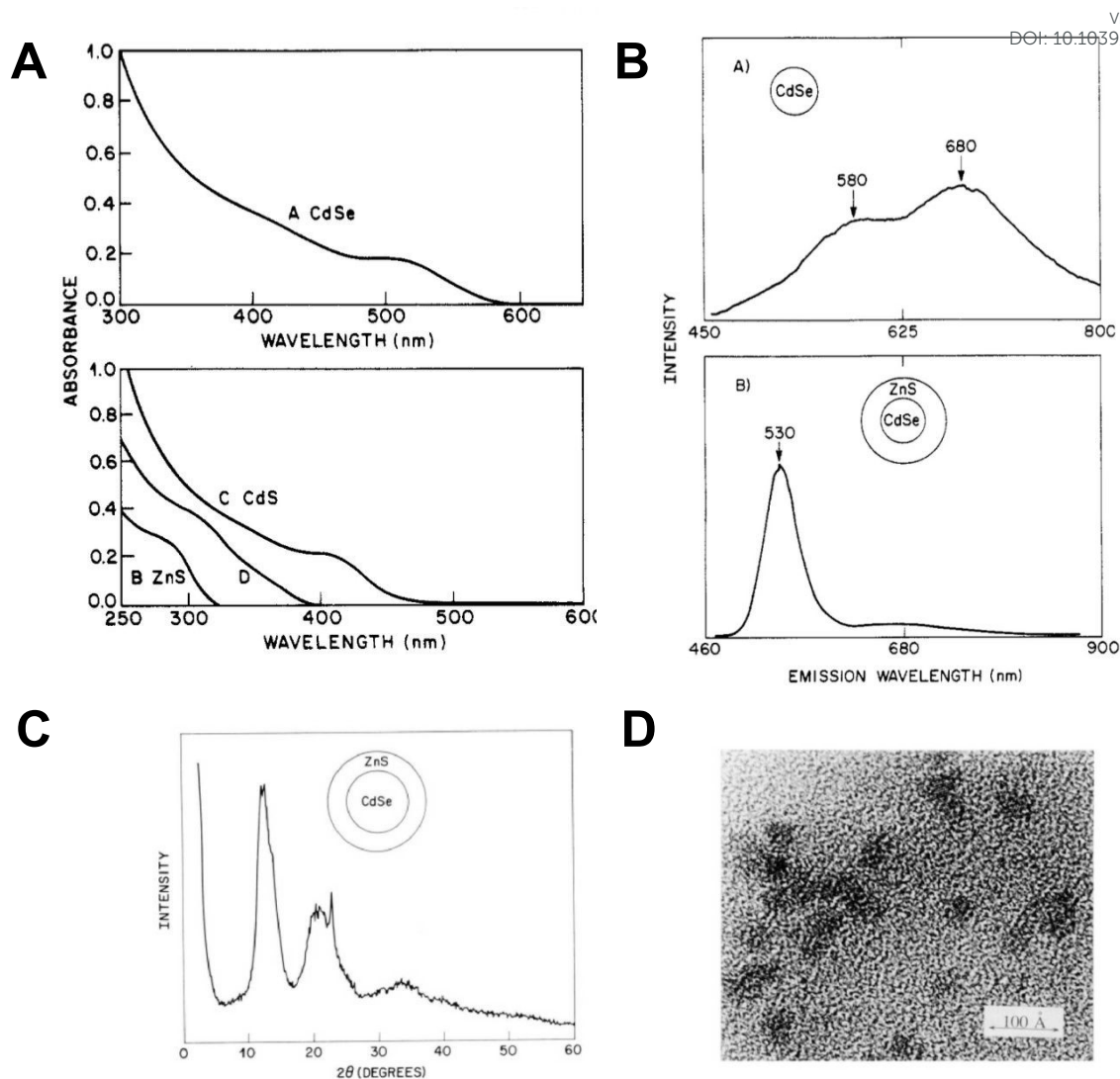
Figure 2 – A) Absorption spectra of A CdSe quantum dots showing excitonic shoulder. B ZnS particles made in a micelle. C CdS particles made in a similar fashion and D product of a ZnS particle reacted with a Cd ion, possibly producing an alloy. B) Room temperature emission spectra of A CdSe particles with a phenyl surface and B (\text{CdSe})_1(\text{ZnS})_4\text{Ph} , which might be described as CdSe/ZnS core/shell quantum dots with a phenyl passivated surface. C) X-ray powder diffraction pattern from (\text{CdSe})_1(\text{ZnS})_4\text{Ph} . D) Electron microscope image of (\text{ZnS})_1(\text{CdSe})_4\text{Ph} quantum dots, which might now be described as an inverse core/shell with a phenyl passivated surface, scale bar = 10 nm. All particles prepared as described in reference 5. Reprinted (adapted) with permission from A. R. Kortan, R. Hull, R. L. Opila, M. G. Bawendi, M. L. Steigerwald, P. J. Carroll, L. E. Brus, J. Am. Chem. Soc. , 1990, 112 , 1327 – 1332. Copyright 2024, American Chemical Society.
