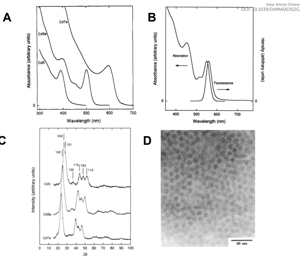
Figure 3 – A) Absorption spectra of CdS, CdSe, and CdTe quantum dots produced by the thermolysis of inorganic and organometallic precursors in tri-n-octylphosphine oxide. B) Absorption and emission spectra of CdSe quantum dots, displaying a blue shifted band edge with discrete energy levels and near band edge emission. C) X-ray diffraction patterns from a selection of CdS, CdSe and CdTe quantum dots. D) Electron micrograph image of CdSe quantum dots, scale bar = 20 nm. All particles prepared as described in reference 1. Reprinted (adapted) with permission from C. B. Murray, D. J. Norris, M. G. Bawendi, J. Am. Chem. Soc. , 1993, 115 , 8706 – 8715. Copyright 2024, American Chemical Society.
