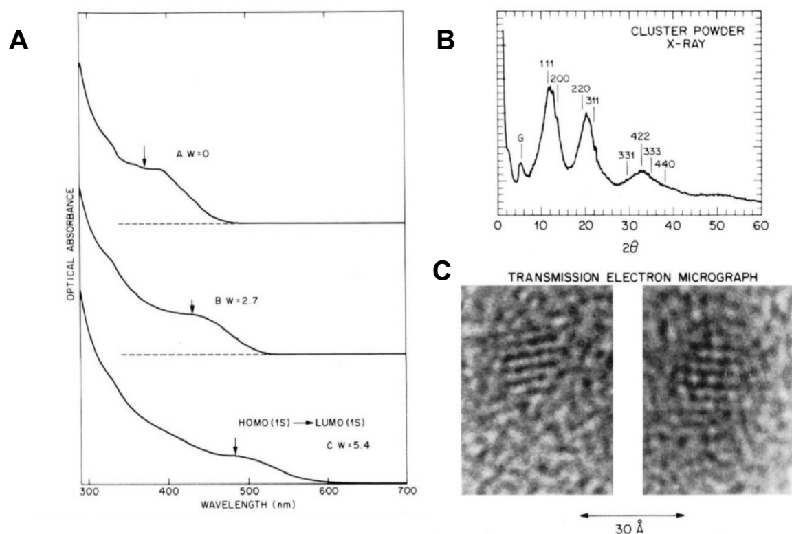
Figure 1 – A) Absorption spectra of CdSe nanocrystals prepared by varying synthesis conditions, showing differing blue shifted band edges and hence different sizes. B) X-ray powder diffraction of CdSe nanoparticles. C) Electron microscope image of CdSe nanoparticles, scale bar = 3 nm. All particles prepared by the micelle methods as described in reference 4. Reprinted (adapted) with permission from M. L. Steigerwald, A. P. Alivisatos, J. M. Gibson, T. D. Harris, R. Kortan, A. J. Muller, A. M. Thayer, T. M. Duncan, D. C. Douglass, L. E. Brus, J. Am. Chem. Soc. , 1988, 110 , 3046 – 3050. Copyright 2024, American Chemical Society.
