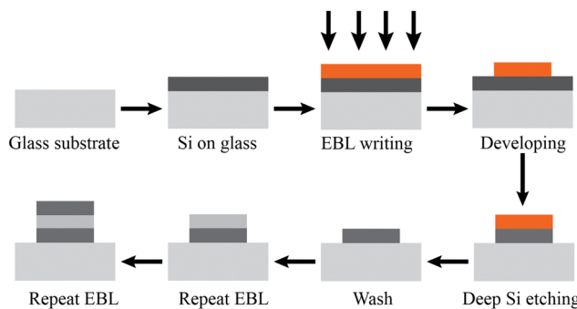
Fig. 11 Suggested fabrication procedure of our proposed dielectric metasurface.
