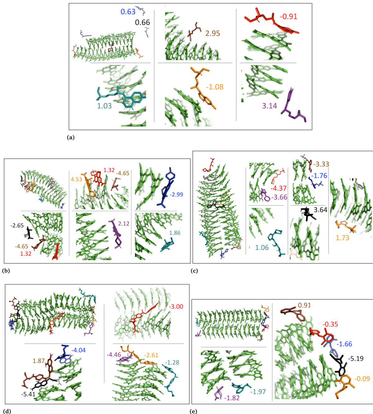
Fig. 5 Illustration shows aggregated DHICAs with charged drug molecules. (a) Chloroquine, (b) levofloxacin, (c) timolol, (d) methotrexate, and (e) diclofenac. Binding energies are shown in kcal mol -1 .
